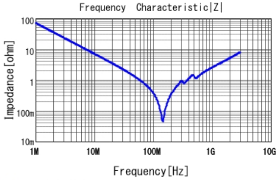
■ GRM21A7U2E222JW31 |Z| DCOV, 25degC
