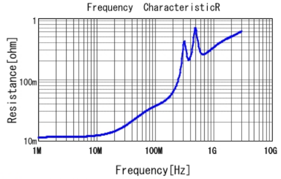
■ GRM21A7U2E222JW31 R DCOV, 25degC
