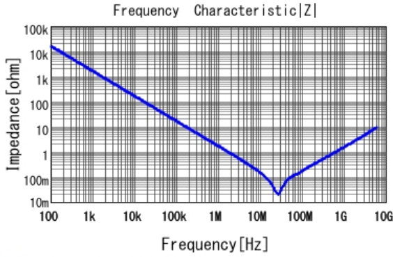
■ GRT155R71C104KE01 |Z| DC0V, 25degC
