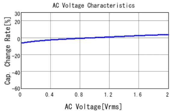
■ GRT155R71C104KE01 C-AC Voltage capchange, DC0V, 25.0d
