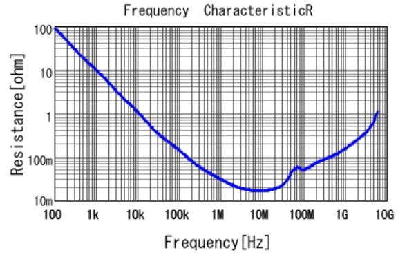
■ GRT155R71C104KE01 R DC0V, 25degC
