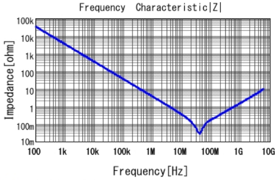
■ GCM155L81C473KA37 |Z| DCOV, 25degC
