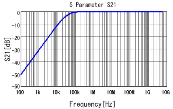
■ GCM155L81C473KA37 S21 DC0V, 25degC
