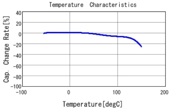
■ GCM155L81C473KA37 C-Temp. capchange, DC0.0V, AC1.0Vrm
