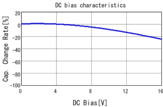
■ GCM155L81C473KA37 C-DC bias capchange, 25.0degC, AC1.
