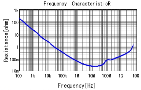
■ GCM155L81C473KA37 R DCOV, 25degC
