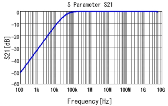
■ GCJ188R92A473KA01 S21 DC0V, 25degC
