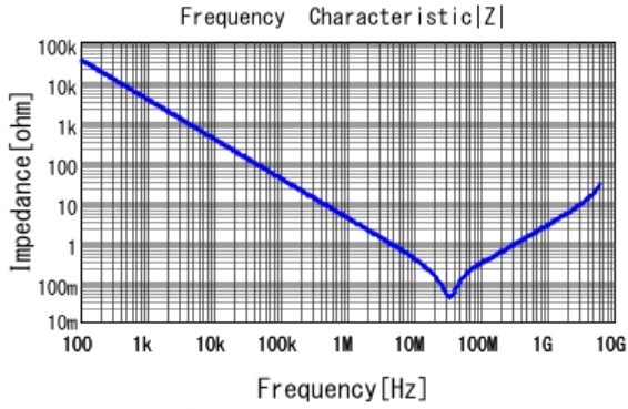
■ GCJ188R92A473KA01 |Z| DCOV, 25degC
