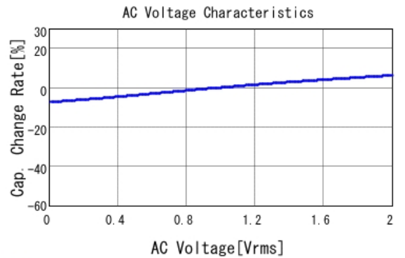
■ GCJ188R92A473KA01 C-AC Voltage capchange, DCOV, 25.0d
