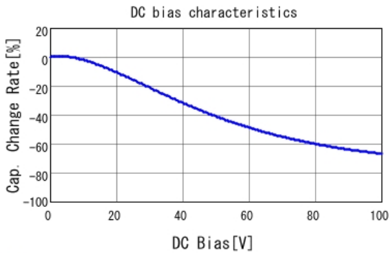
■ GCJ188R92A473KA01 C-DC bias capchange, 25.0degC, AC1.
