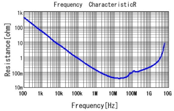
■ GCJ188R92A473KA01 R DCOV, 25degC
