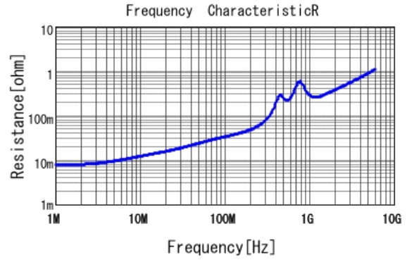
■ GRM2165C2A182JA01 R DCOV, 25degC
