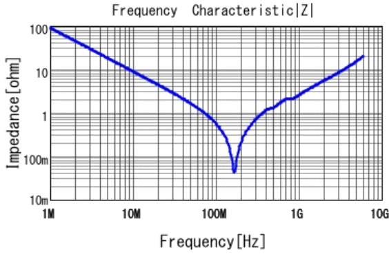
■ GRM2165C2A182JA01 |Z| DCOV, 25degC
