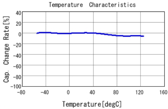
■ GCJ188R71E102KA01 C-Temp. capchange, DC0.0V, AC1.0Vrm
