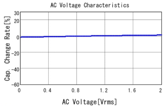
■ GCJ188R71E102KA01 C-AC Voltage capchange, DCOV, 25.0d
