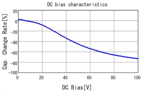
GCM155R72A472KA37 C-DC bias capchange, 25.0degC, AC1.
