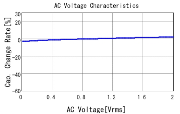
GCM155R72A472KA37 C-AC Voltage capchange, DC0V, 25.0d
