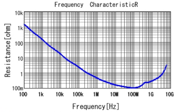
GCM155R72A472KA37 R DC0V, 25degC
