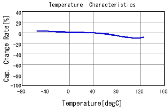
■ GCM155R72A472KA37 C-Temp. capchange, DC0.0V, AC1.0Vrm
