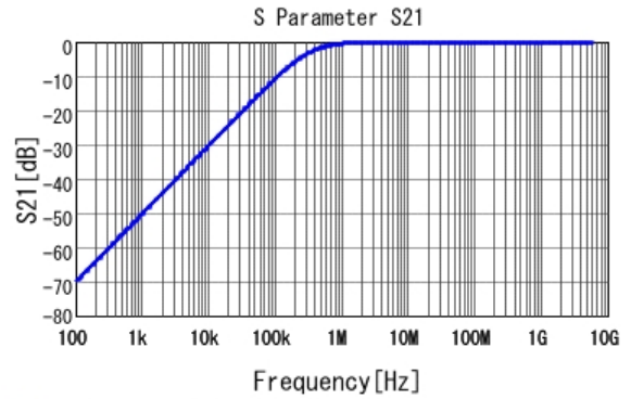
■ GCM155R72A472KA37 S21 DC0V, 25degC
