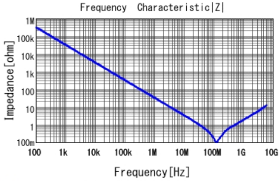
GCM155R72A472KA37 |Z| DC0V, 25degC
