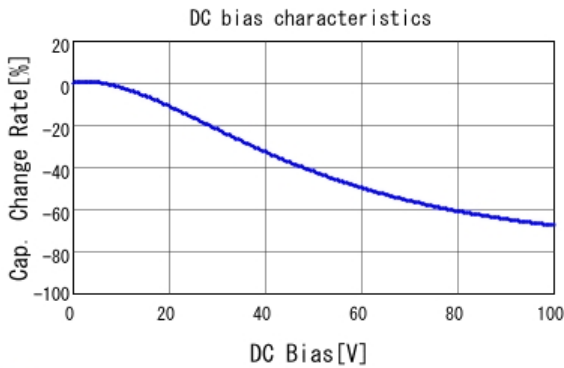
■ GCJ188R92A683KA01 C-DC bias capchange, 25.0degC, AC1.
