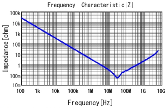
■ GCJ188R92A683KA01 |Z| DCOV, 25degC
