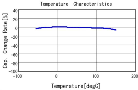
■ GCJ188R92A683KA01 C-Temp. capchange, DC0.0V, AC1.0Vrm
