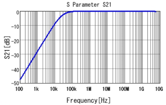
■ GCJ188R92A683KA01 S21 DC0V, 25degC
