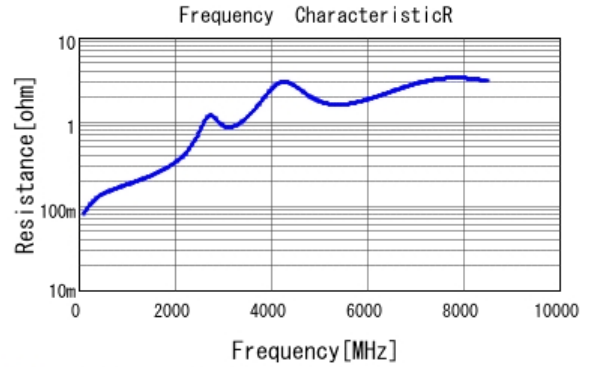
■ GCM1555C1H470JA16 R DCOV, 25degC
