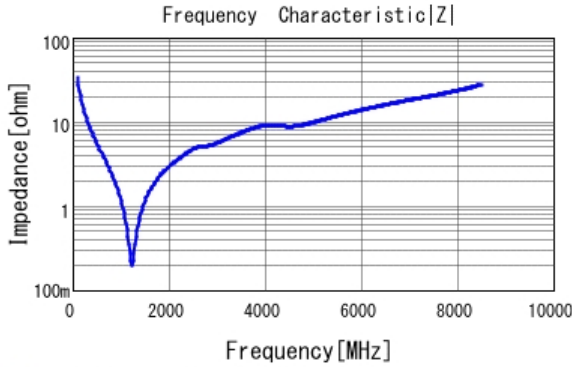
■ GCM1555C1H470JA16 |Z| DCOV, 25degC
