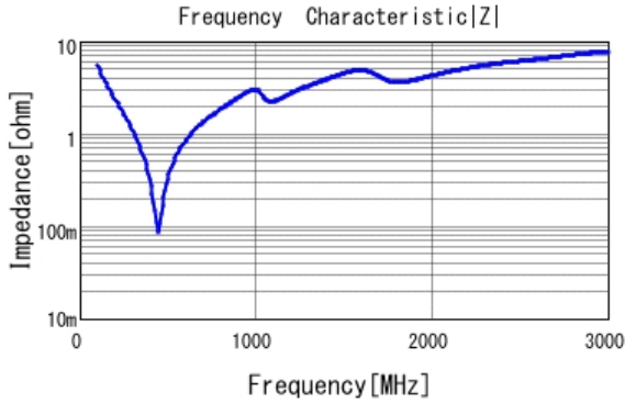
■ GRM21A5C2E271JW01 |Z| DC0V, 25degC
