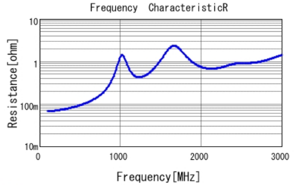
■ GRM21A5C2E271JW01 R DC0V, 25degC
