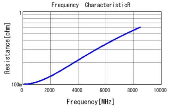
■ GJM1555C1H5R6CB01 R DC0V, 25degC
