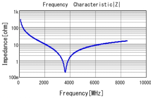
■ GJM1555C1H5R6CB01 |Z| DC0V, 25degC
