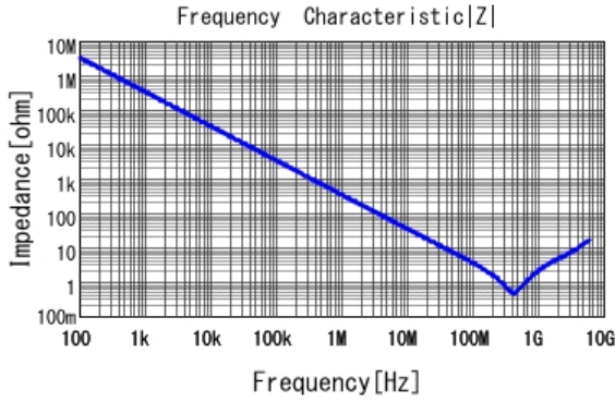
■ GRM155R72A471KA01 |Z| DCOV, 25degC
