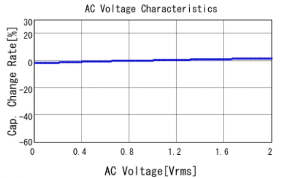
■ GRM155R72A471KA01 C-AC Voltage capchange, DCOV, 25.0d
