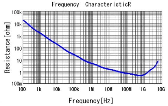
■ GRM155R72A471KA01 R DCOV, 25degC
