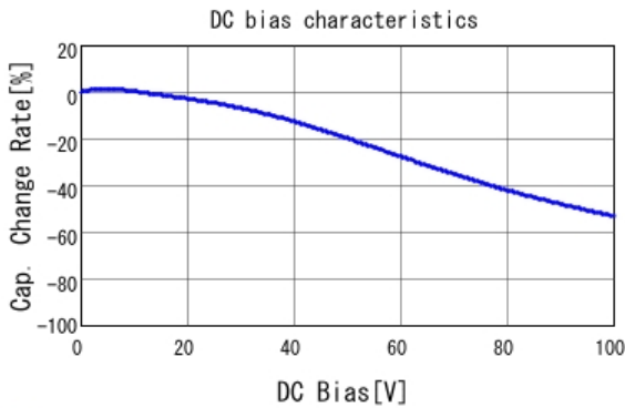
■ GRM155R72A471KA01 C-DC bias capchange, 25.0degC, AC1.
