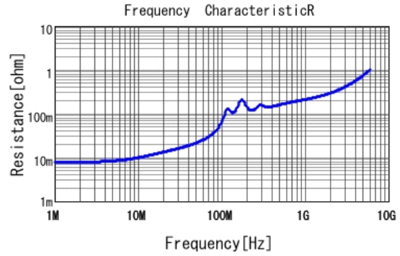
■ GRM1887U1A153JA01 R DCOV, 25degC
