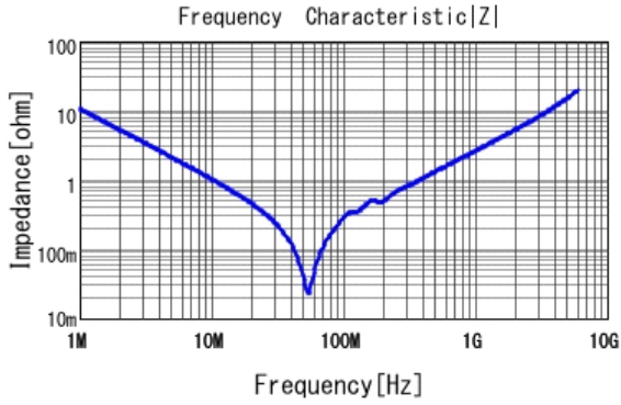
■ GRM1887U1A153JA01 |Z| DCOV, 25degC
