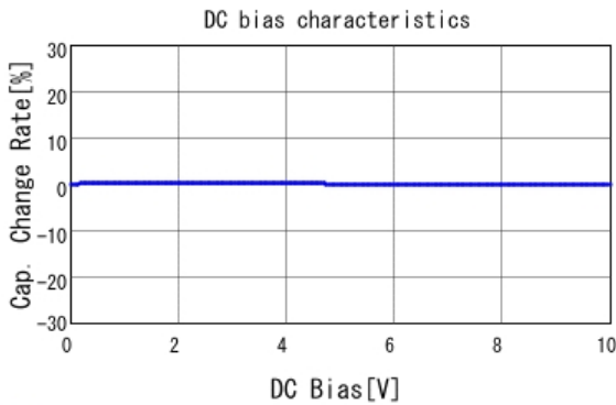
■ GRM1887U1A153JA01 C-DC bias capchange, 25.0degC, AC1V
