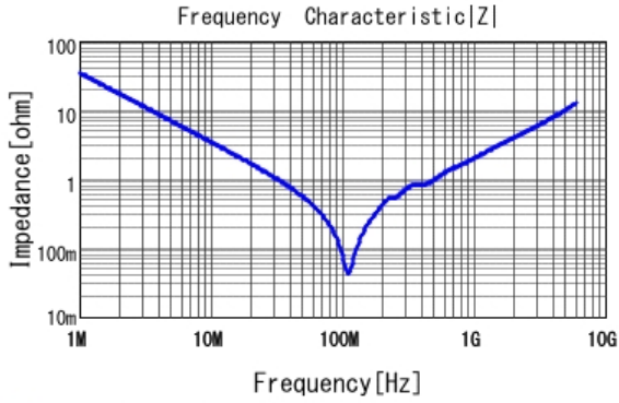
■ GRM1857U1H472JA44 |Z| DCOV, 25degC
