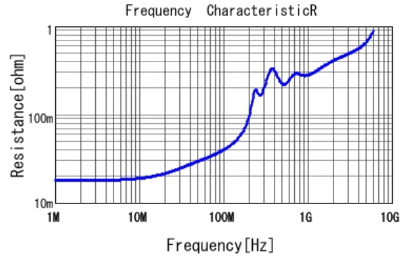
■ GRM1857U1H472JA44 R DCOV, 25degC
