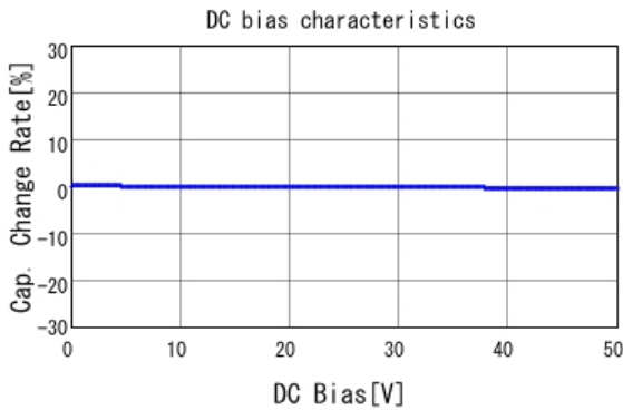
■ GRM1857U1H472JA44 C-DC bias capchange, 25.0degC, AC1V
