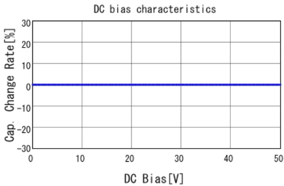
■ GRM1885C1H272JA01 C-DC bias capchange, 25.0degC, AC1V
