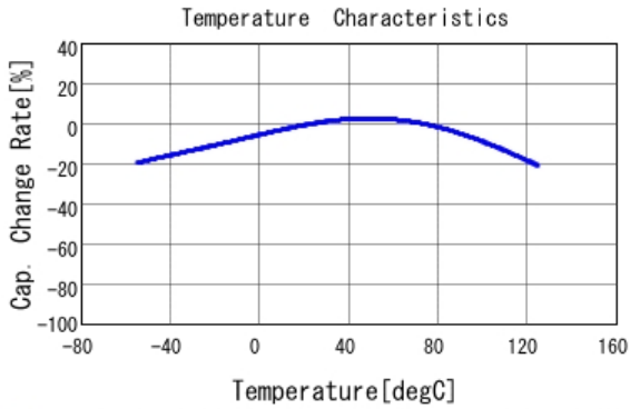
GCM21BC7YA475KE36 C-Temp. capchange, DC0.0V, AC0.5Vrm
