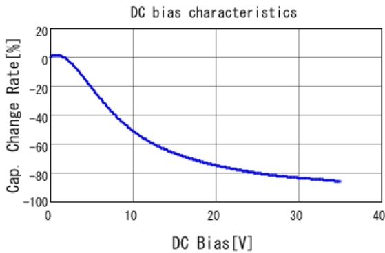
■ GCM21BC7YA475KE36 C-DC bias capchange, 25.0degC, AC1V
