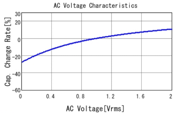
■ GCM21BC7YA475KE36 C-AC Voltage capchange, DC0V, 25.0d
