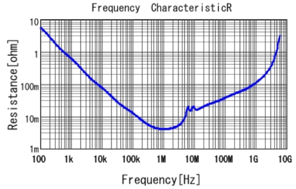
■ GCM21BC7YA475KE36 R DC0V, 25degC
