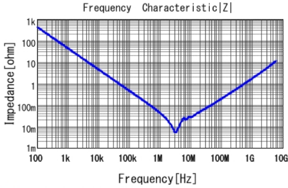
■ GCM21BC7YA475KE36 |Z| DC0V, 25degC
