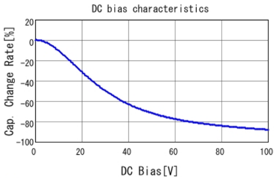
■ GRJ21BC72A105KE11 C-DC bias capchange, 25.0degC, AC1.
