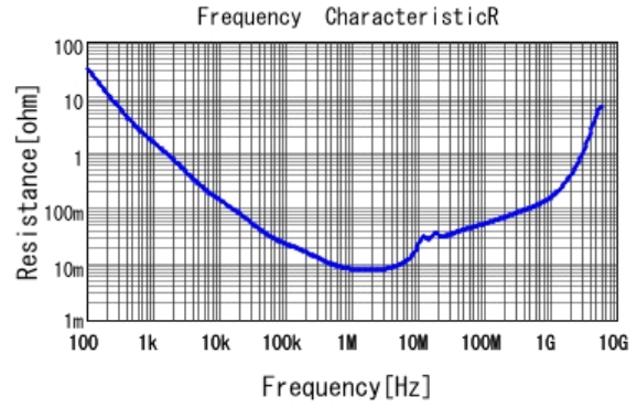
■ GRJ21BC72A105KE11 R DC0V, 25degC
