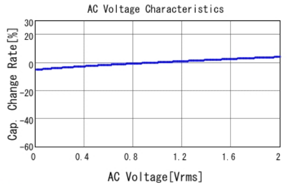
■ GRJ21BC72A105KE11 C-AC Voltage capchange, DC0V, 25.0d
