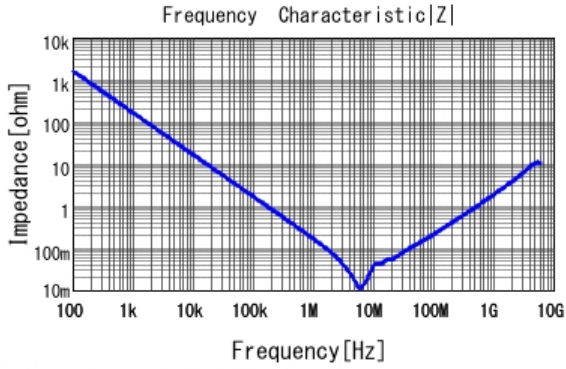
■ GRJ21BC72A105KE11 |Z| DC0V, 25degC
