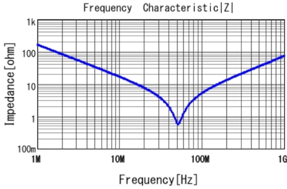
■ DE1E3RA102MA4BQ01F |Z| DCOV, 20degC
