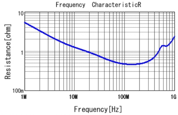
■ DE1E3RA102MA4BQ01F R DCOV, 20degC
