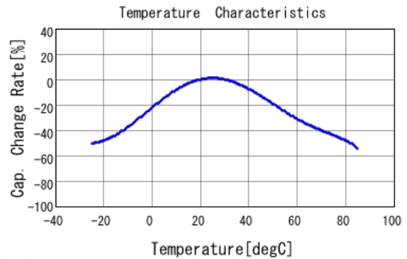
■ DE1E3RA102MA4BQ01F C-Temp. capchange, DCOV, AC1Vrms
