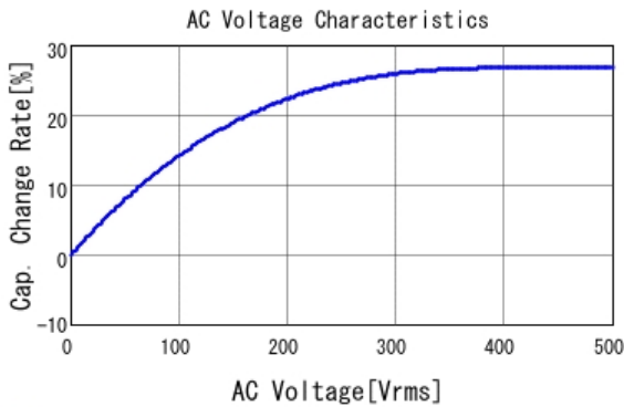
■ DE1E3RA102MA4BQ01F C-AC Voltage capchange, DCOV, 20.0
