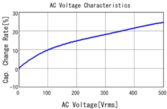
■ DE1B3RA331KA4BQ01F C-AC Voltage capchange, DCOV, 20.0
