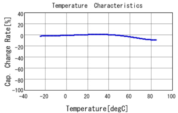
■ DE1B3RA331KA4BQ01F C-Temp. capchange, DCOV, AC1Vrms
