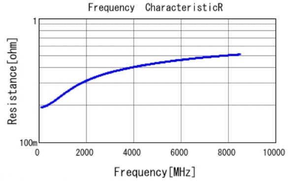
■ GRM0225C1E3R2CA03 R DCOV, 25degC
