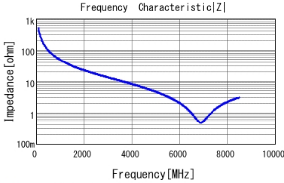
■ GRM0225C1E3R2CA03 |Z| DCOV, 25degC
