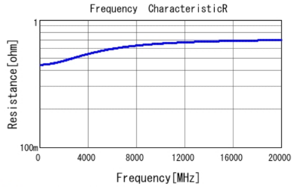
■ GRM0225C1H1R1WA03 R DCOV, 25degC
