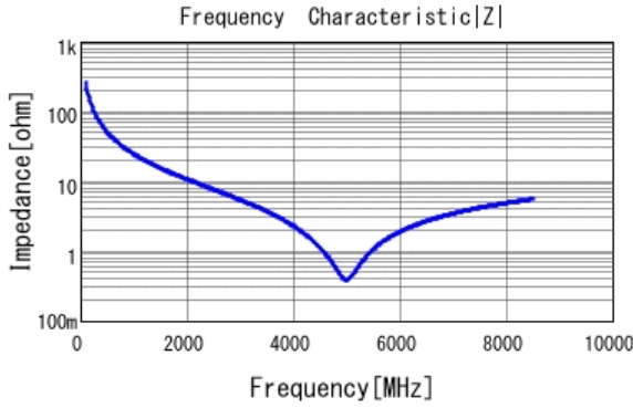
■ GRM0225C1E6R2CA03 |Z| DCOV, 25degC
