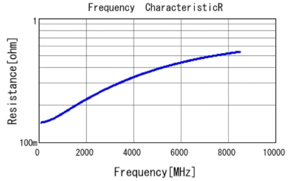
■ GRM0225C1E6R2CA03 R DCOV, 25degC
