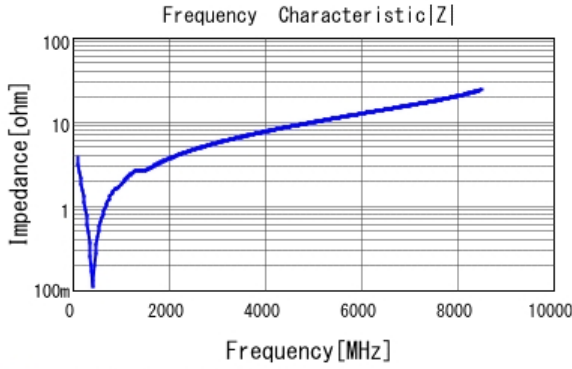
■ GRM1555C1H391JA01 |Z| DCOV, 25degC
