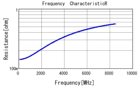
■ GRM0225C1E7R2CA03 R DCOV, 25degC
