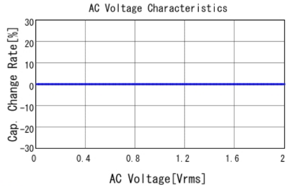
■ GRM0225C1E7R2CA03 C-AC Voltage capchange, DCOV, 25.0d
