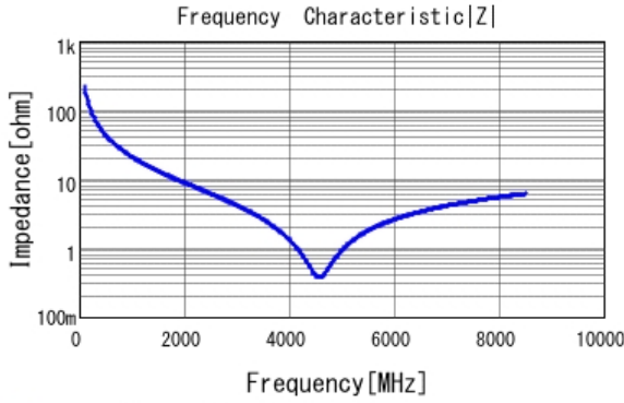
■ GRM0225C1E7R2CA03 |Z| DCOV, 25degC
