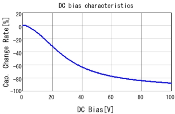
■ GRM21BC72A105KE01 C-DC bias capchange, 25.0degC, AC1.
