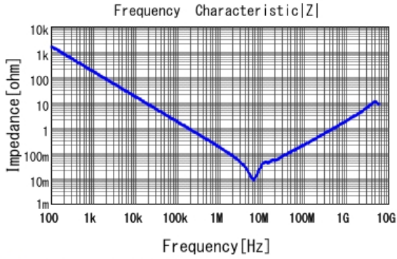
■ GRM21BC72A105KE01 |Z| DCOV, 25degC
