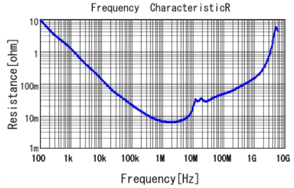
■ GRM21BC72A105KE01 R DCOV, 25degC
