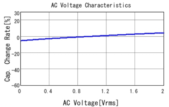
■ GRM21BC72A105KE01 C-AC Voltage capchange, DCOV, 25.0d
