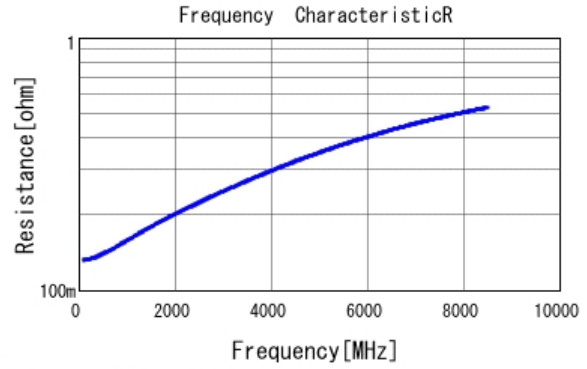
■ GRM0225C1E9R2CA03 R DC0V, 25degC
