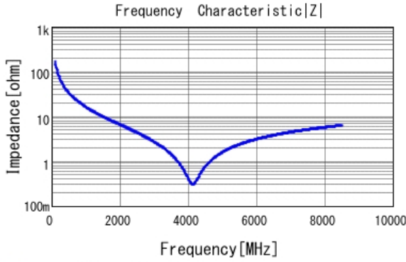
■ GRM0225C1E9R2CA03 |Z| DC0V, 25degC
