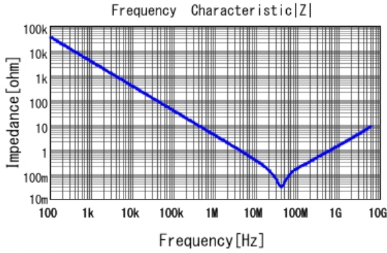
GCM155R71H473KE02 |Z| DC0V, 25degC
