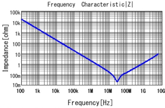
■ GRM155R71E104KE14 |Z| DCOV, 25degC
