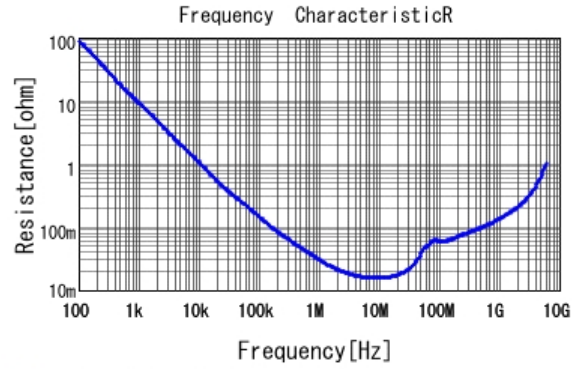
■ GRM155R71E104KE14 R DCOV, 25degC
