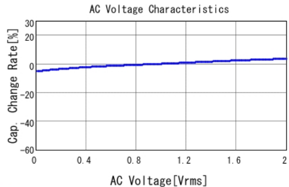
■ GRM155R71H104KE14 C-AC Voltage capchange, DC0V, 25.0d
