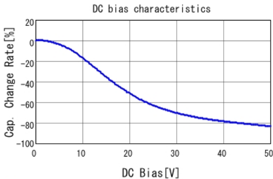
■ GRM155R71H104KE14 C-DC bias capchange, 25.0degC, AC1.
