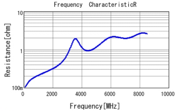
■ GCM1555C1H270JA16 R DCOV, 25degC
