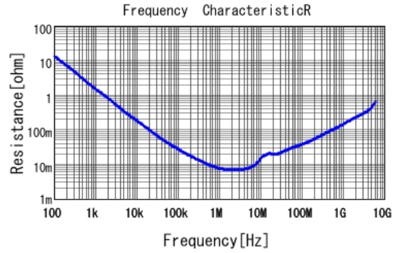
■ GRM155C70J225KE11 R DCOV, 25degC
