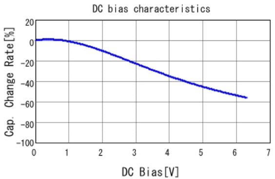
■ GRM155C70J225KE11 C-DC bias capchange, 25.0degC, AC0.
