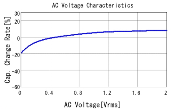
■ GRM155C70J225KE11 C-AC Voltage capchange, DCOV, 25.0d
