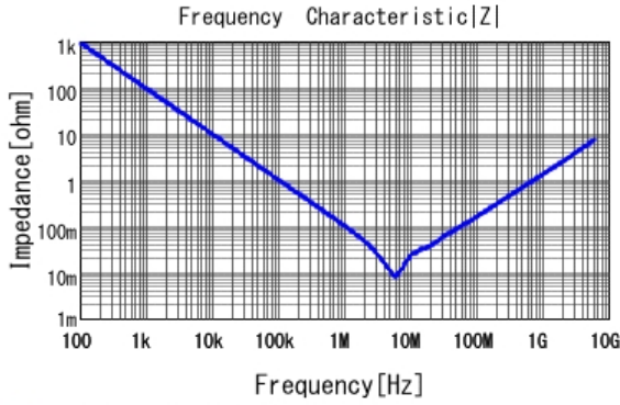
■ GRM155C70J225KE11 |Z| DCOV, 25degC
