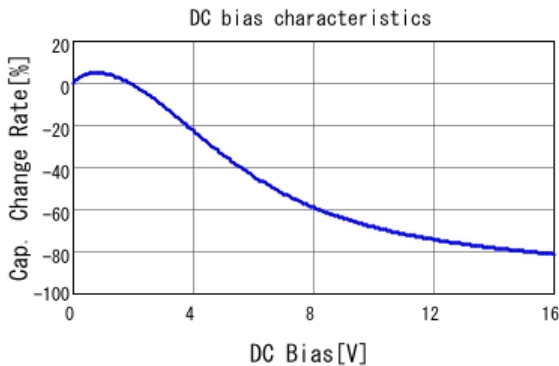
GCM155R71C224KE02 C-DC bias capchange, 25.0degC, AC1.
