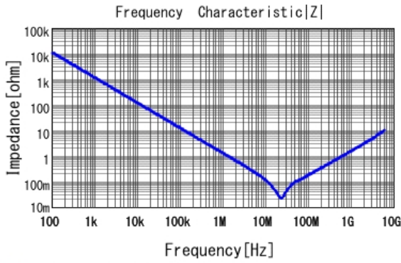
GCM155R71C224KE02 |Z| DC0V, 25degC
