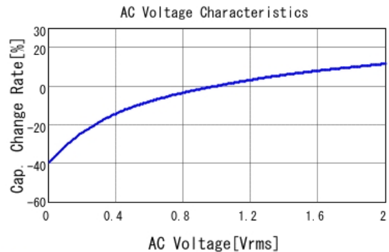
GCM155R71C224KE02 C-AC Voltage capchange, DC0V, 25.0d
