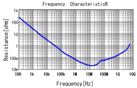
GCM155R71C224KE02 R DC0V, 25degC
