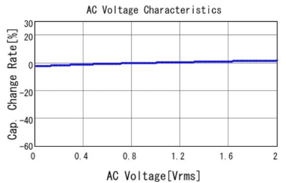
■ GCJ21BR72A473KA01 C-AC Voltage capchange, DCOV, 25.0d
