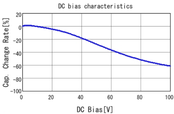
■ GCJ21BR72A473KA01 C-DC bias capchange, 25.0degC, AC1.
