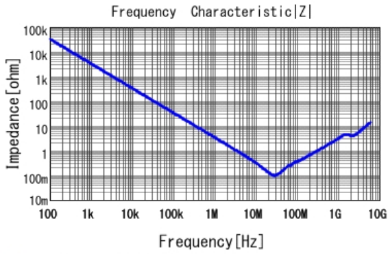
■ GCJ21BR72A473KA01 |Z| DCOV, 25degC
