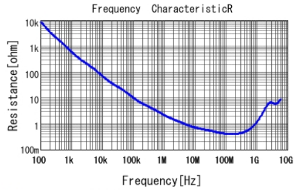
■ GCJ188R72A102KA01 R DCOV, 25degC
