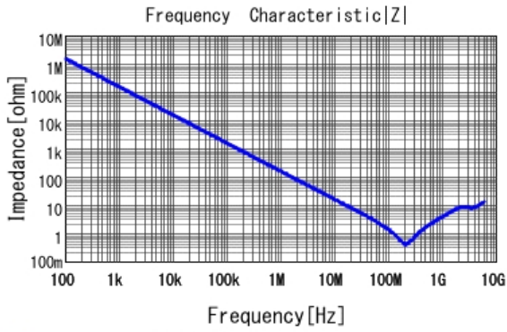
■ GCJ188R72A102KA01 |Z| DCOV, 25degC
