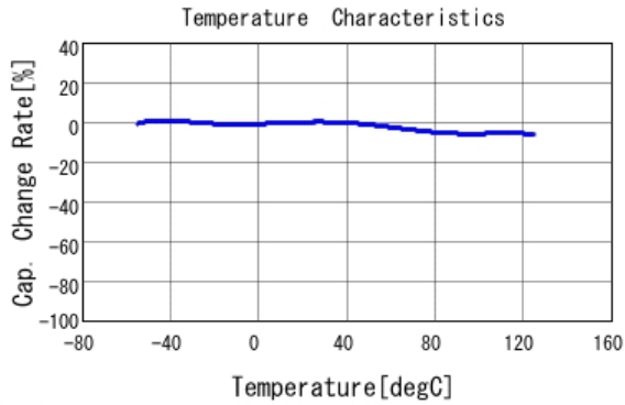
■ GCJ188R72A102KA01 C-Temp. capchange, DC0.0V, AC1.0Vrm
