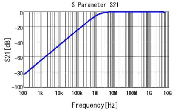
■ GCJ188R72A102KA01 S21 DC0V, 25degC
