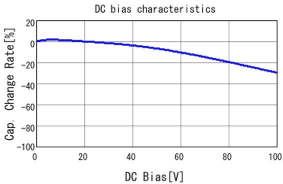
■ GCJ188R72A102KA01 C-DC bias capchange, 25.0degC, AC1.
