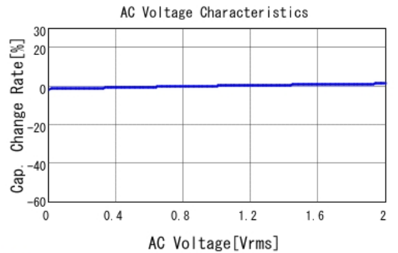
■ GCJ188R72A102KA01 C-AC Voltage capchange, DCOV, 25.0d
