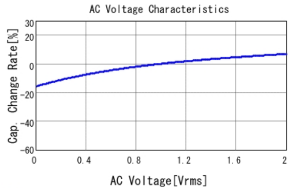
■ GCJ188R91E474KA01 C-AC Voltage capchange, DCOV, 25.0d
