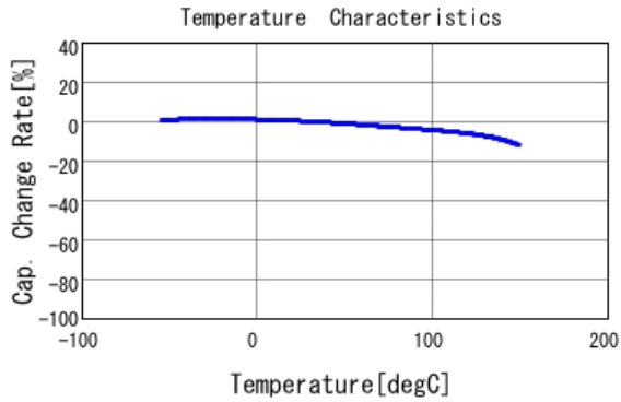
■ GCJ188R91E474KA01 C-Temp. capchange, DC0.0V, AC1.0Vrm
