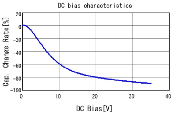
■ GRM188C8YA225KE11 C-DC bias capchange, 25.0degC, AC1V
