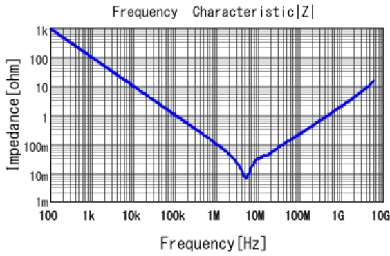
■ GRM188C8YA225KE11 |Z| DCOV, 25degC
