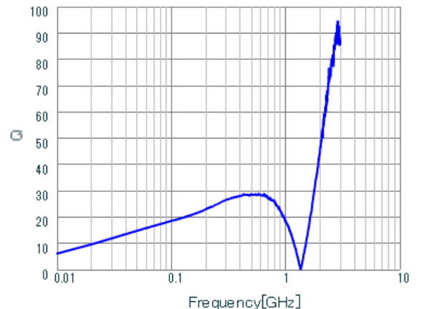
Q-Frequency Characteristics
