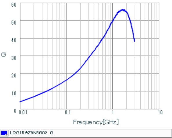
Q-Frequency Characteristics
