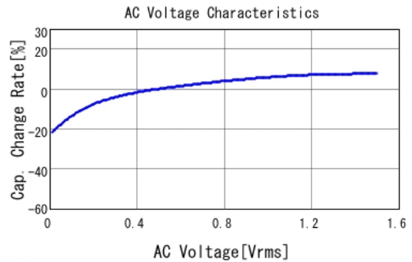
ZRA21CR61E226ME01 C-AC Voltage capchange, DC0V, 25.0d
