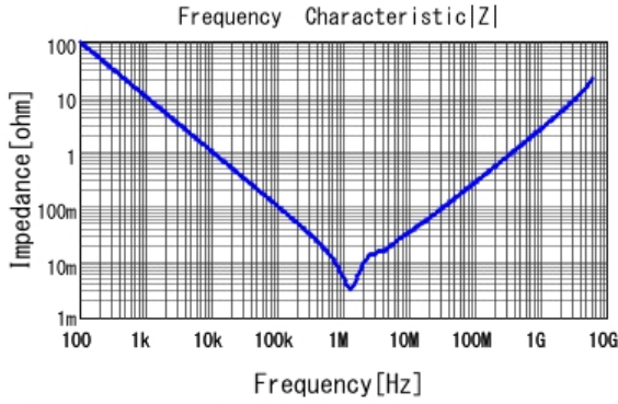
ZRA21CR61E226ME01 |Z| DC0V, 25degC
