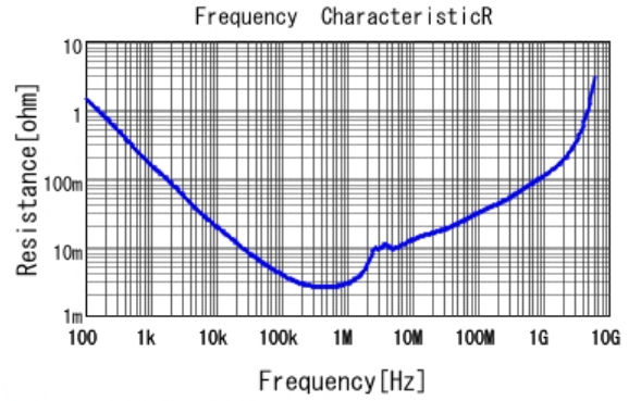
ZRA21CR61E226ME01 R DC0V, 25degC
