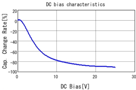
ZRA21CR61E226ME01 C-DC bias capchange, 25.0degC, AC0.
