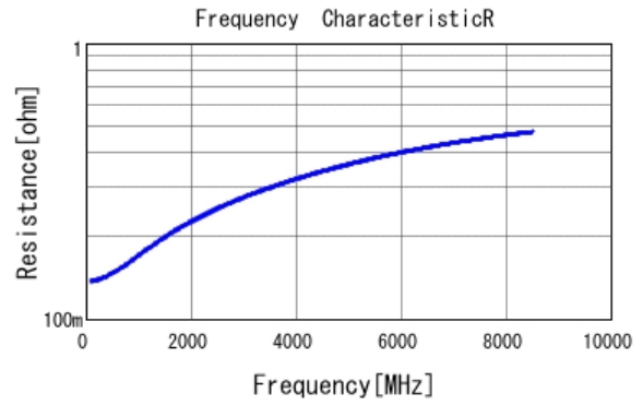
■ GRM0225C1H8R2WA03 R DCOV, 25degC
