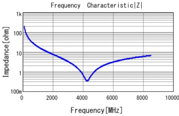
■ GRM0225C1H8R2WA03 |Z| DCOV, 25degC
