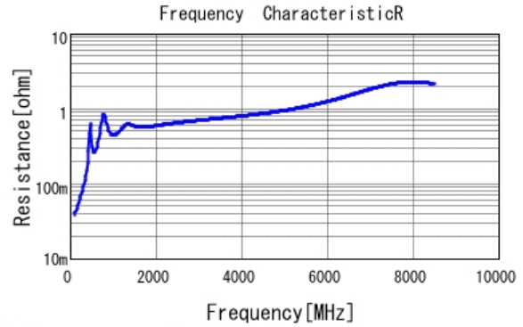
■ GCM1885C2A821JA16 R DCOV, 25degC
