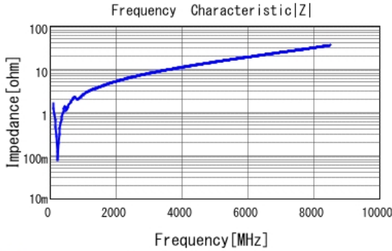
■ GCM1885C2A821JA16 |Z| DCOV, 25degC
