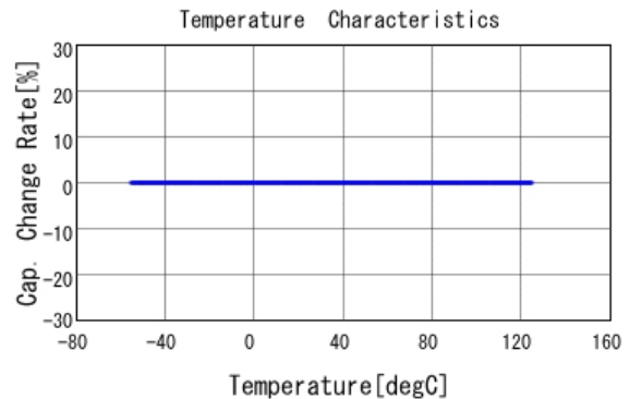
■ GRM21A5C2E821JWA1 C-Temp. capchange, DCOV, AC1Vrms
