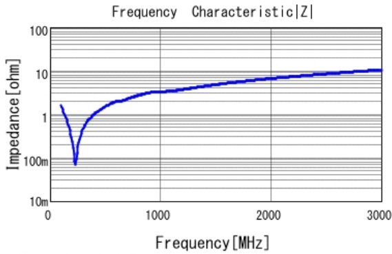
■ GRM21A5C2E821JWA1 |Z| DCOV, 25degC
