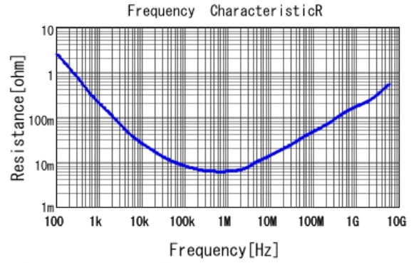
ZRB15XR60J106ME12 R DC0V, 25degC
