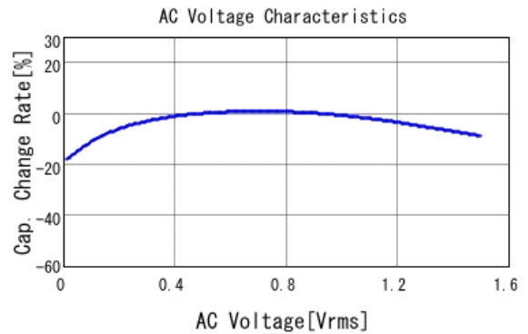
ZRB15XR60J106ME12 C-AC Voltage capchange, DC0V, 25.0d
