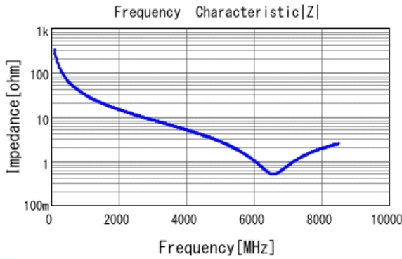
■ GRM0115C1E5R0CE01 |Z| DCOV, 25degC
