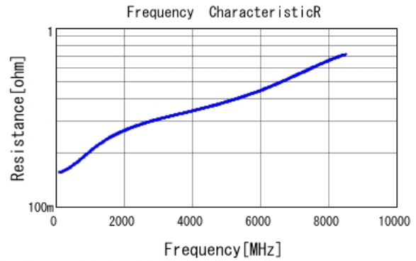
■ GRM0115C1E5R0CE01 R DCOV, 25degC
