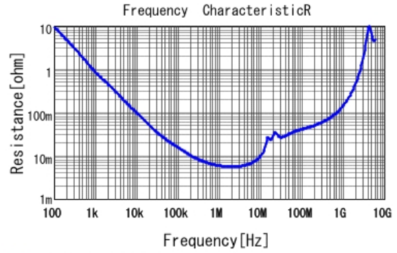
GCM21BR7YA684KA55 R DCOV, 25degC
