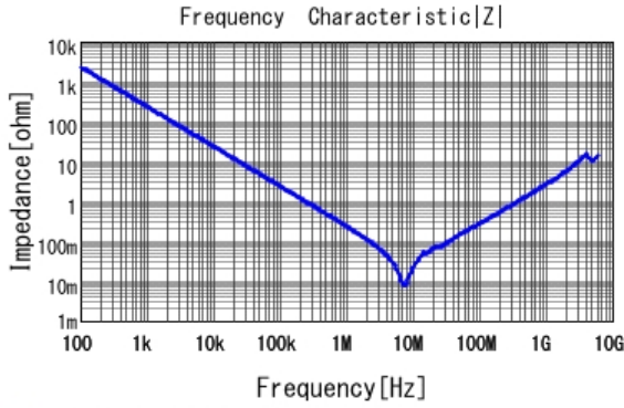
GCM21BR7YA684KA55 |Z| DCOV, 25degC
