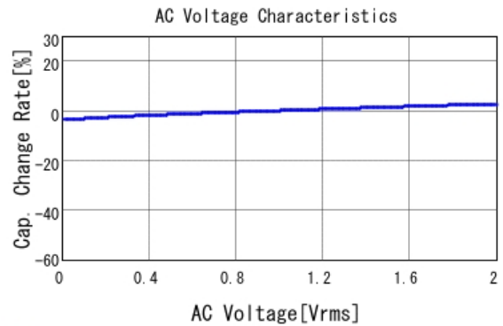
GCM21BR7YA684KA55 C-AC Voltage capchange, DCOV, 25.0d
