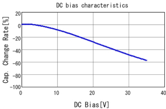
GCM21BR7YA684KA55 C-DC bias capchange, 25.0degC, AC1.
