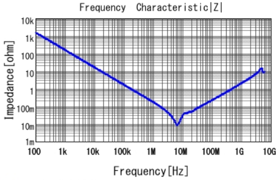
GCM21BR71E155KA54 |Z| DC0V, 25degC
