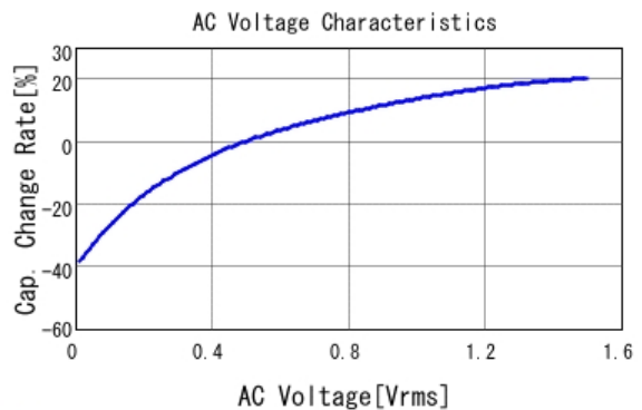
■ GCM21BR70J106KE22 C-AC Voltage capchange, DCOV, 25.0d
