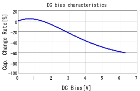
■ GCM21BR70J106KE22 C-DC bias capchange, 25.0degC, AC0.
