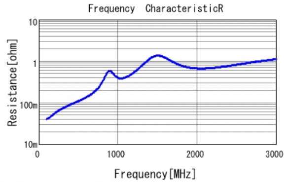
■ GRM21A5C2E391JWA1 R DCOV, 25degC
