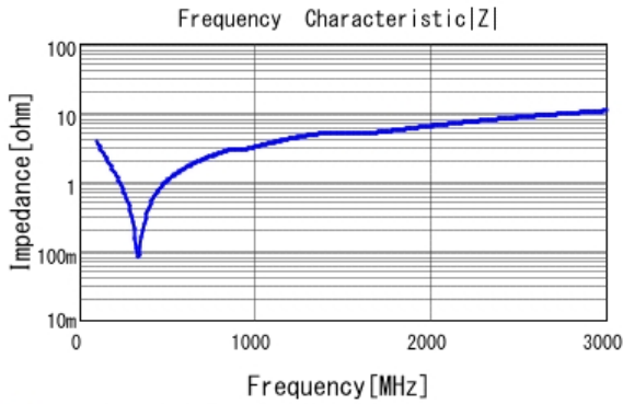
■ GRM21A5C2E391JWA1 |Z| DCOV, 25degC
