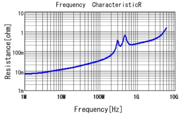
■ GRM2165C2A272JA01 R DCOV, 25degC
