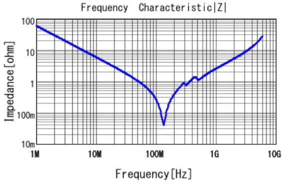
■ GRM2165C2A272JA01 |Z| DCOV, 25degC
