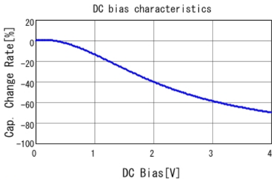
■ GRM219R60G476ME44 C-DC bias capchange, 25.0degC, AC0.
