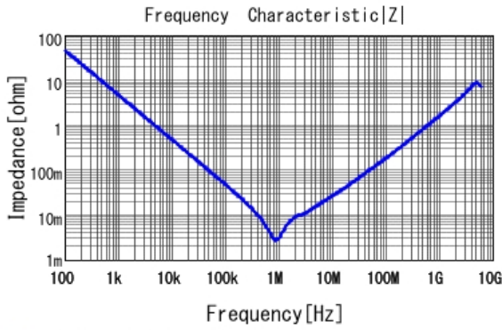
■ GRM219R60G476ME44 |Z| DCOV, 25degC
