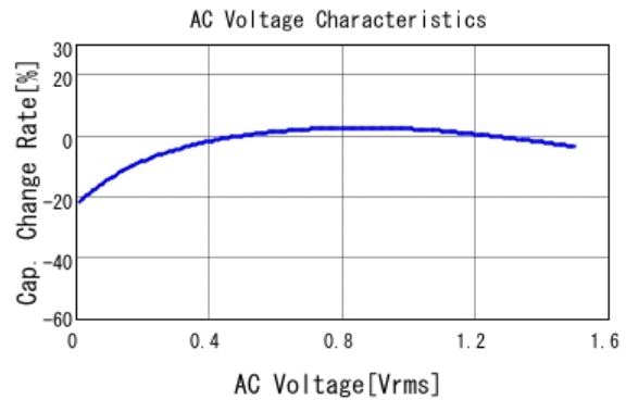
■ GRM219R60G476ME44 C-AC Voltage capchange, DCOV, 25.0d
