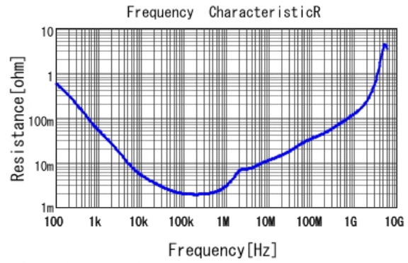
■ GRM219R60G476ME44 R DCOV, 25degC
